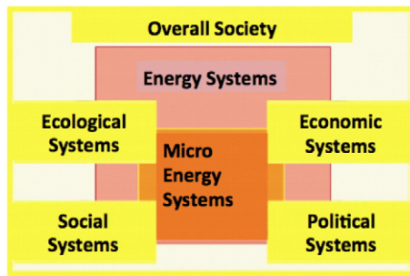
Fig. 1. Definition of microenergy systems. (Source: Philipp & Schäfer 2009).
